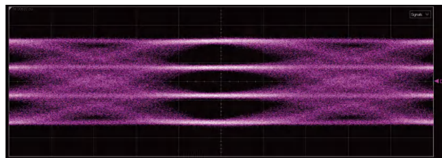
PPG码型发生器输出53.125Gbps 注入LFSJ 100KHz正弦抖动示例
