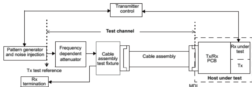
Figure 110-3a—Interference tolerance test setup
